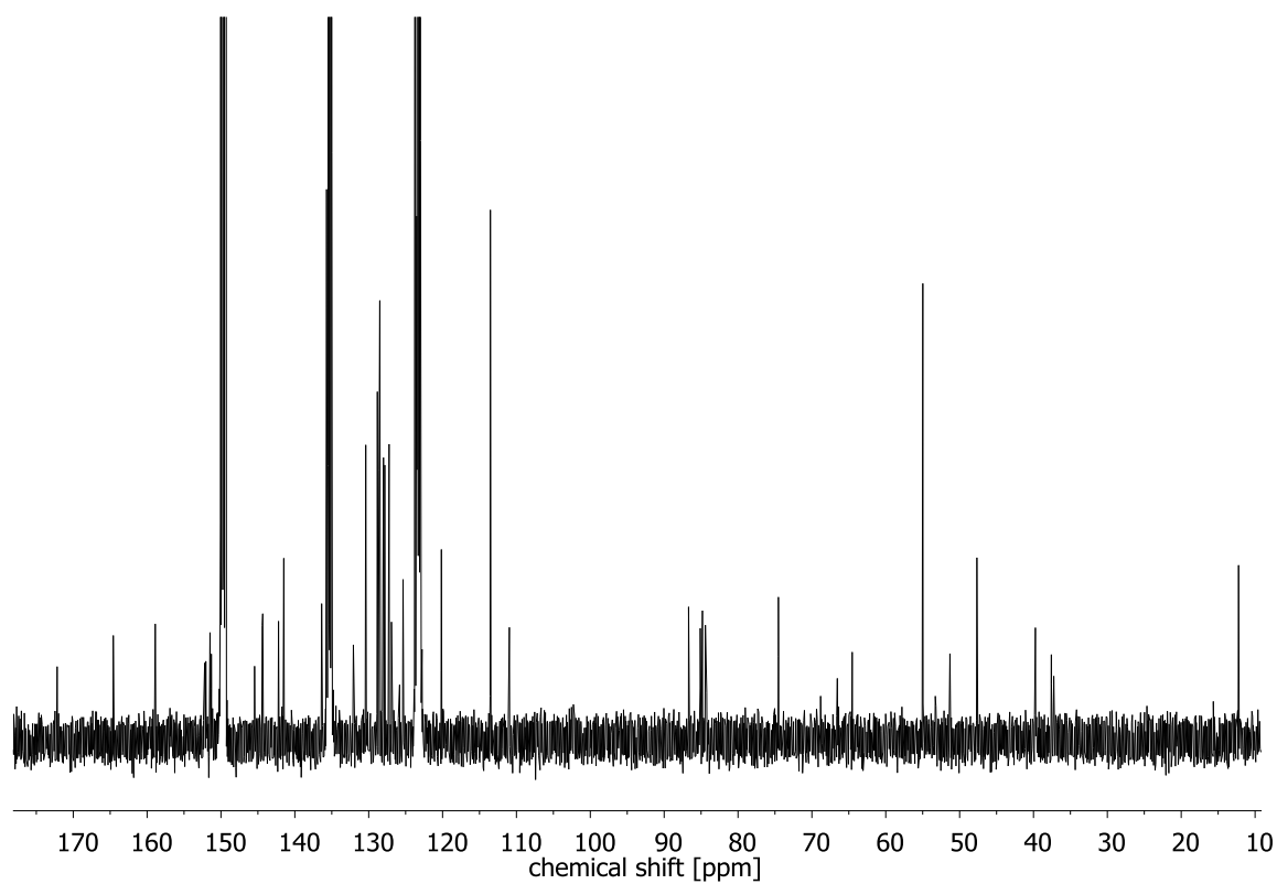
^{13}\text{C} NMR spectrum of ( S )- 28 (126 MHz, pyridine- \text{d}_5 , 50 °C)
