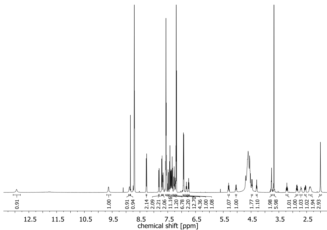
^1\text{H} NMR spectrum of ( S )- 28 (500 MHz, pyridine- \text{d}_5 , 50 °C)
