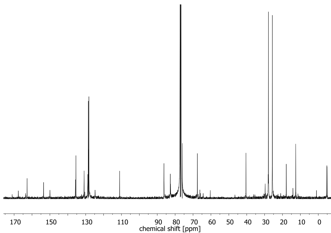
^{13}\text{C} NMR spectrum of Z-18 (75 MHz, \text{CDCl}_3 )
