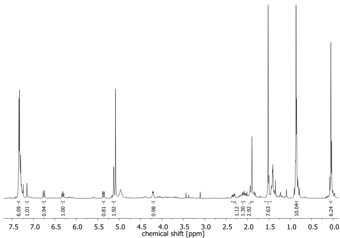
^1\text{H} NMR spectrum of E - 18 (300 MHz, \text{CDCl}_3 )
