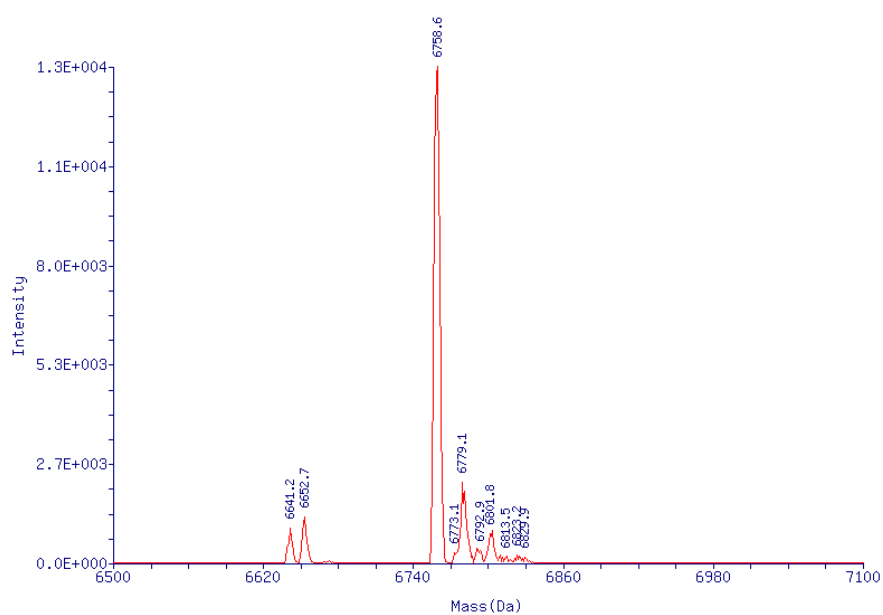
Mass spectrum of 31 (5'-GGCACGGA x T x TTTTGGCACGG-3', x = (6' R )-NAA)
