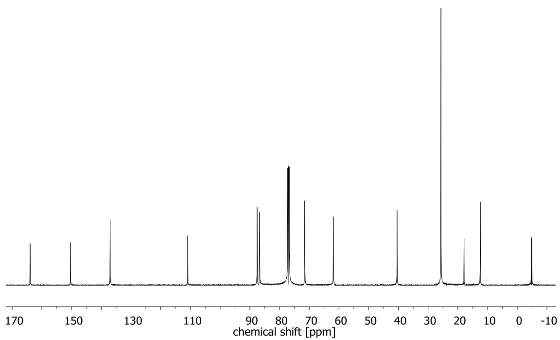
^{13}\text{C} NMR spectrum of 16 (75 MHz, \text{CDCl}_3 )
