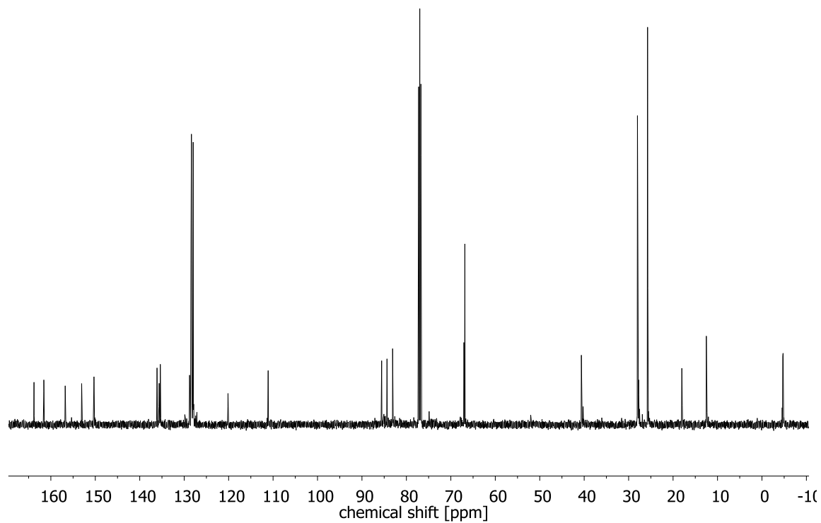
^{13}\text{C} NMR spectrum of E - 18 (75 MHz, \text{CDCl}_3 )
