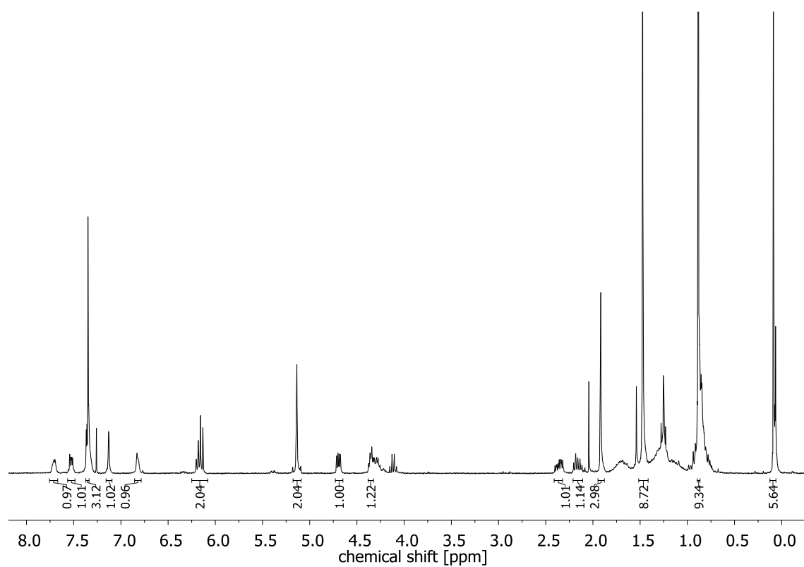
^1\text{H} NMR spectrum of Z-18 (300 MHz, \text{CDCl}_3 )
