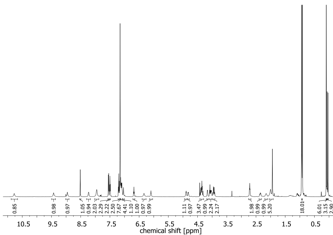
^1\text{H} NMR spectrum of ( S )- 26 (500 MHz, \text{C}_6\text{D}_6 , 70 °C)
