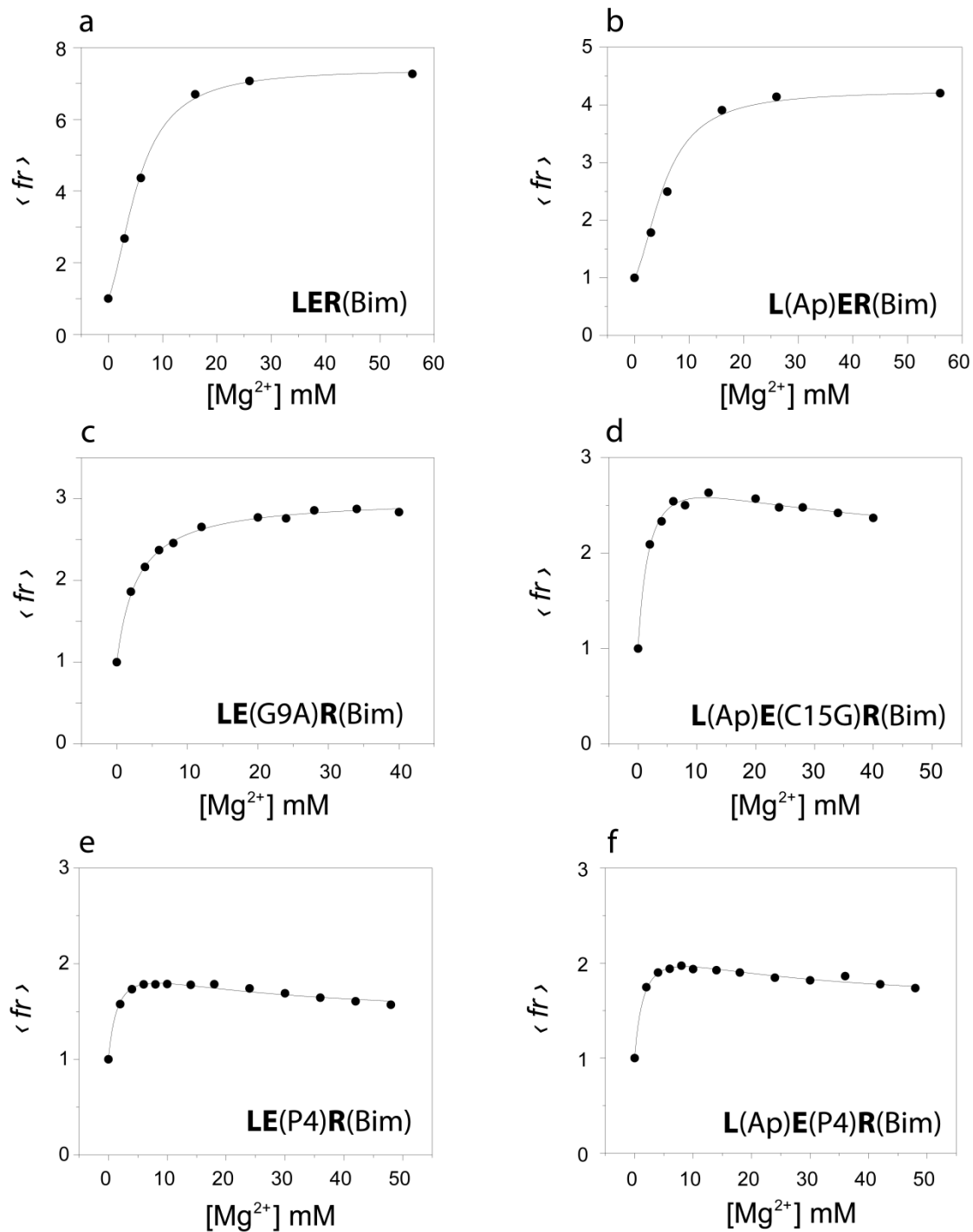
Supplementary Figure S3. Changes in \langle fr \rangle of the complexes L(x)E(y)R(Bim) upon titration with MgCl_2 . 1 \mu M L(x)E(y)R(Bim) , 0-56 mM MgCl_2 , 150 mM NaCl, 2 mM KCl, 50 mM Na-HEPES, pH 7.5; 15 °C; \lambda_{exc} = 398 nm, \lambda_{em} = 480 nm. The titrations were analyzed with the two-step equilibrium model (described in Figure 1 and Equation 6), except for L(Ap)E(G9A)R(Bim) , which was fit to a single step reaction.
