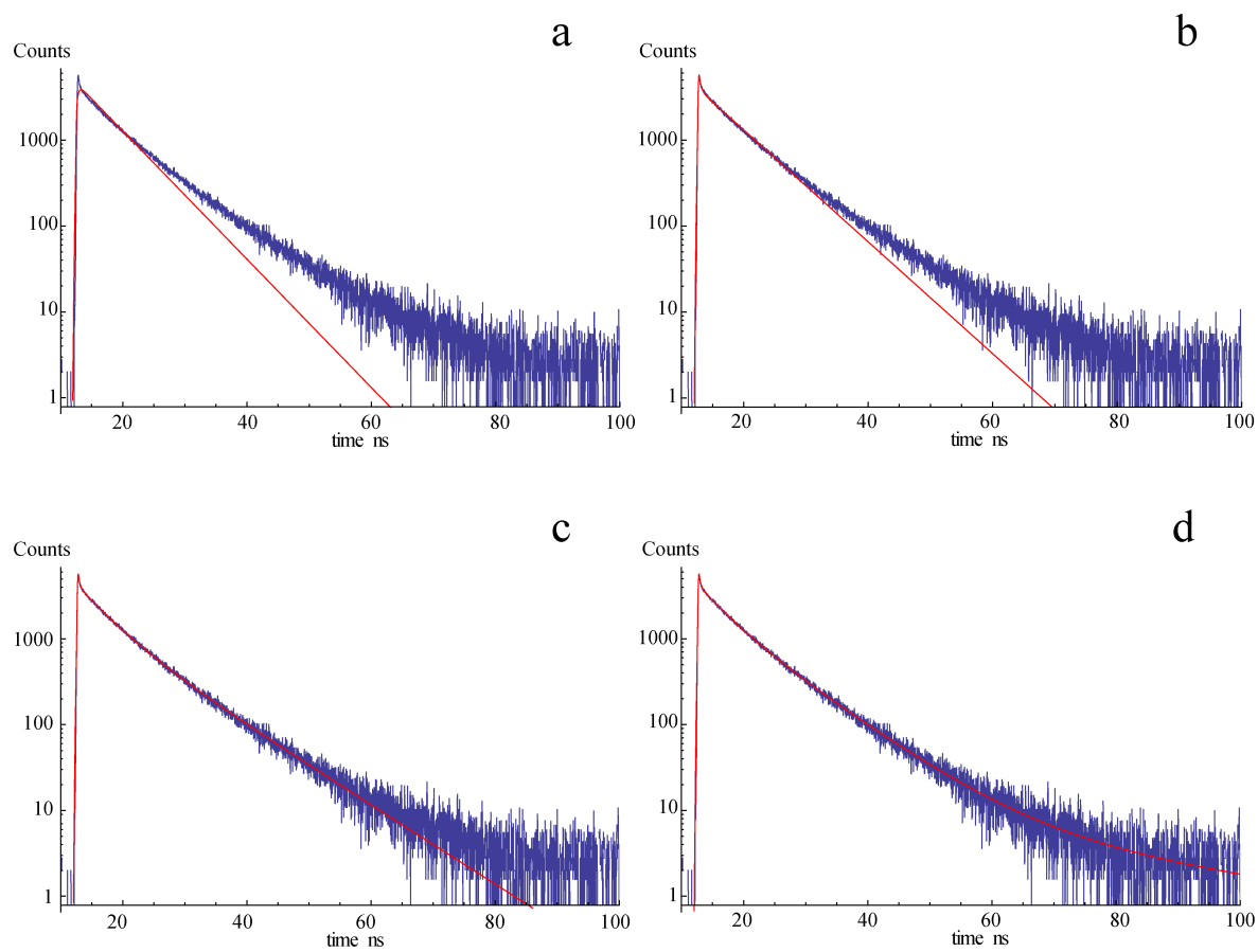
Supplementary Figure S4: Fluorescence decay of L(dAP)ER(Bim). a-d) fits to 1, 2, 3, or 4 exponential components, respectively. Conditions: 4.2 \mu M L(dAp), 4.1 \mu M E, 4.0 \mu M R(Bim).
